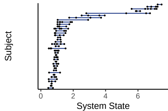
Prevotella_melaninogenica_ε
