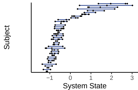
Eubacterium_biforme_et_rel
