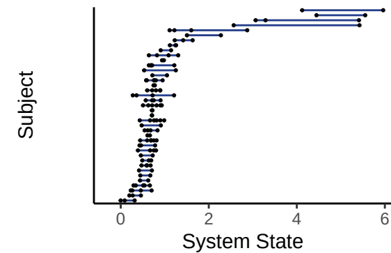
Uncultured_Mollicutes
